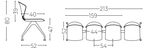
Beam seating Bancada
